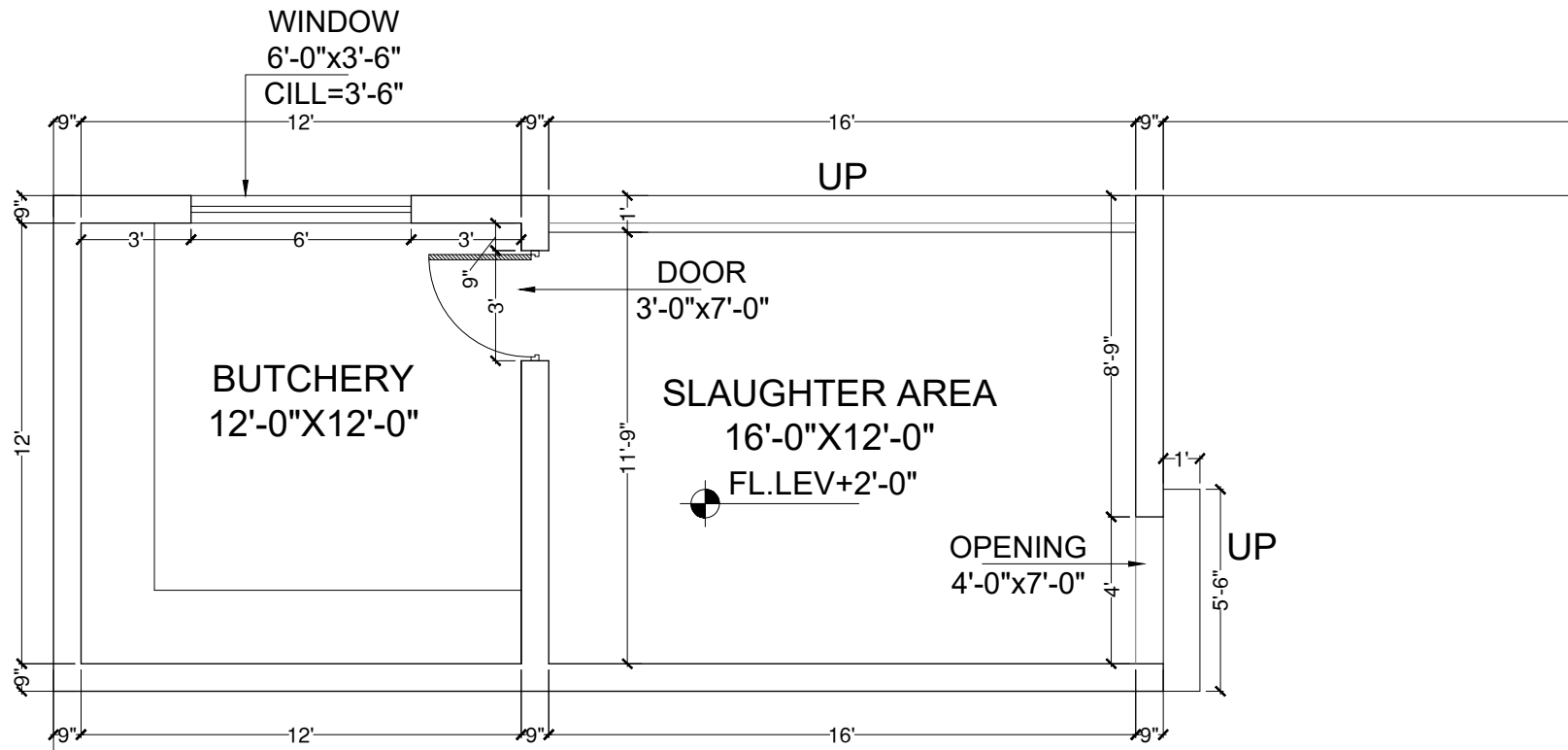
SKAUGHTER AREA LAYOUT PLAN
